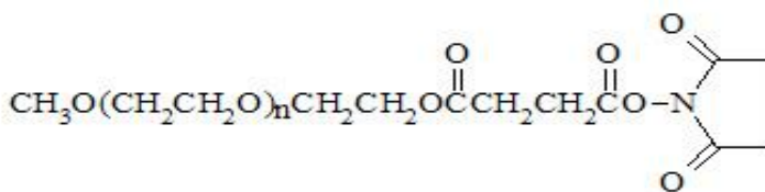
mPEG-SS
