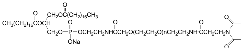
DSPE-PEG-MAL
