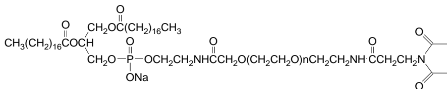
DSPE-PEG-MAL
