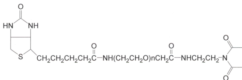
Biotin-PEG-Maleimide
