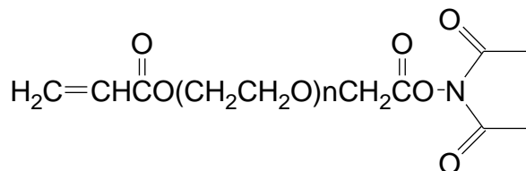
Acrylate-PEG-SCM
