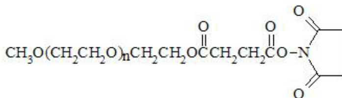
mPEG-SS
