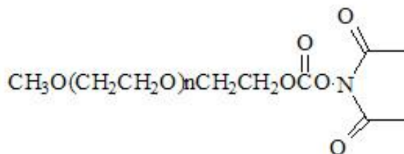
mPEG-SC
