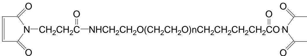
MAL-PEG-SVA
