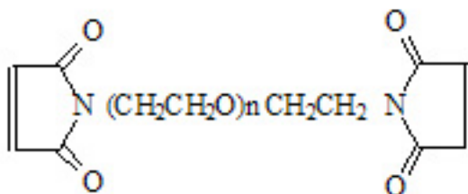
MAL-PEG-MAL
