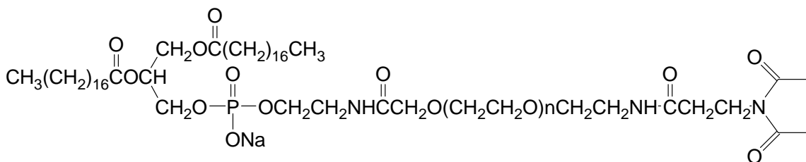
DSPE-PEG-MAL
