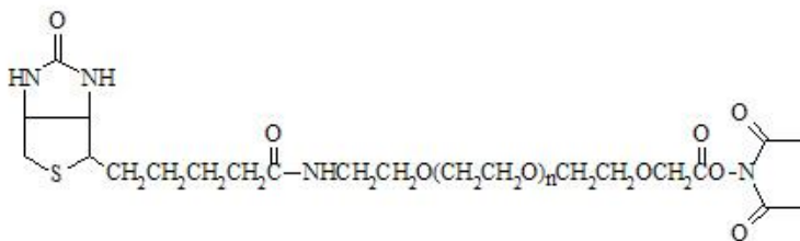
Biotin-PEG-SCM
