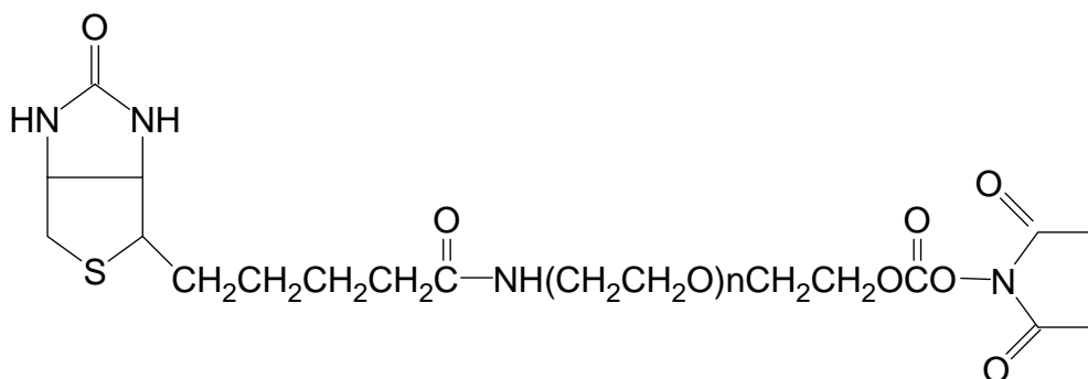
Biotin-PEG-SC
