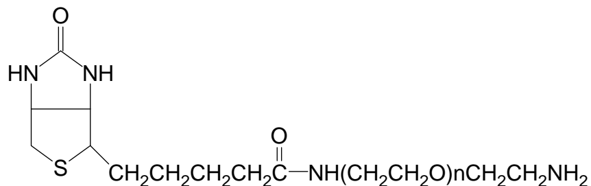
Biotin-PEG-Amine
