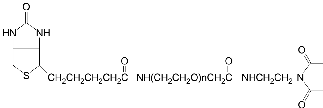
Biotin-PEG-Maleimide
